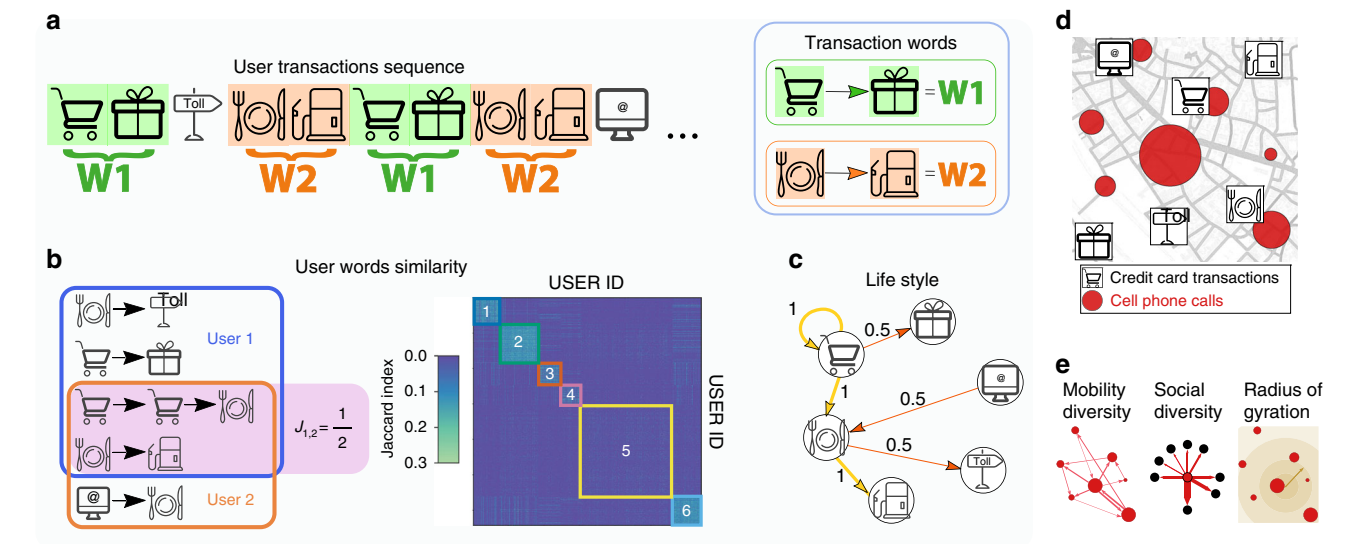
Fig. 2 Methods and metrics. a Schematic representation of the Sequitur's algorithm applied to a sequence of transactions of one user to detect words and identify significant transaction sequences in the data set. b Calculation of the similarity between two users (left) based on the Jaccard index of their significant sequences to define the matrix of users' similarity (right). Group of users are detected based on similar sequences of transactions. c Lifestyle representation based on sample users 1 and 2 of b . d Example of traces of CDR and CCR data for the user. e Metrics adopted for the analysis of CDR data. The icons used in this figure are work of Azaze11o/Shutterstock.com
